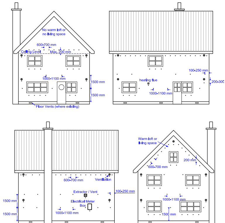
Diagram 2: Partial Fill Drill Pattern
